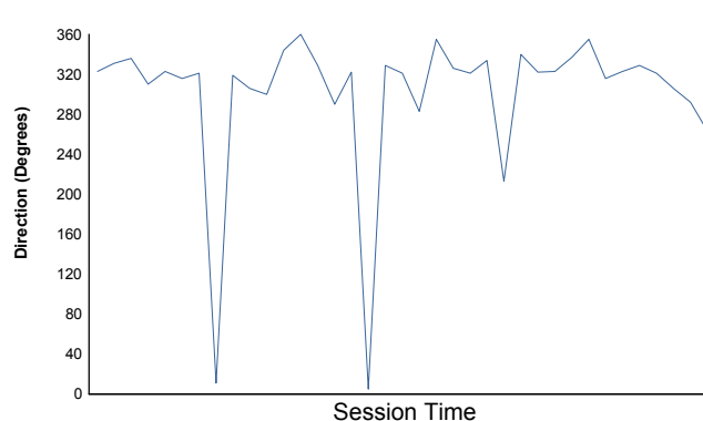
Wind direction
